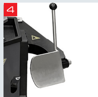
■ Bead breaker for motorcycle wheels with double-acting cylinder and fixed blade .
