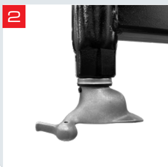
■ Mounting head for motorcycle wheels.
